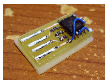
The Undetectable USB CapsLocker Macetech
