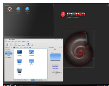
PC-BSD 7.0 PC-BSD
