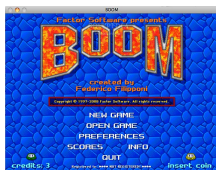
Title screen
